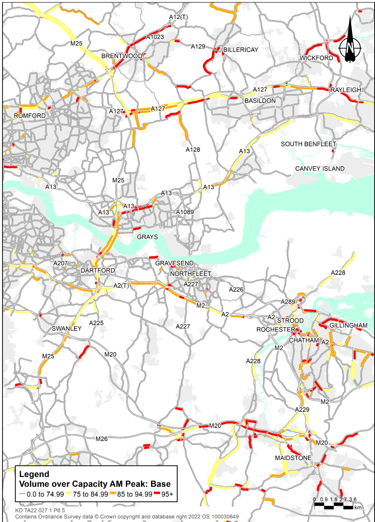
Plate 6.5 Volume to capacity 2016 AM peak (07:00–08:00)
