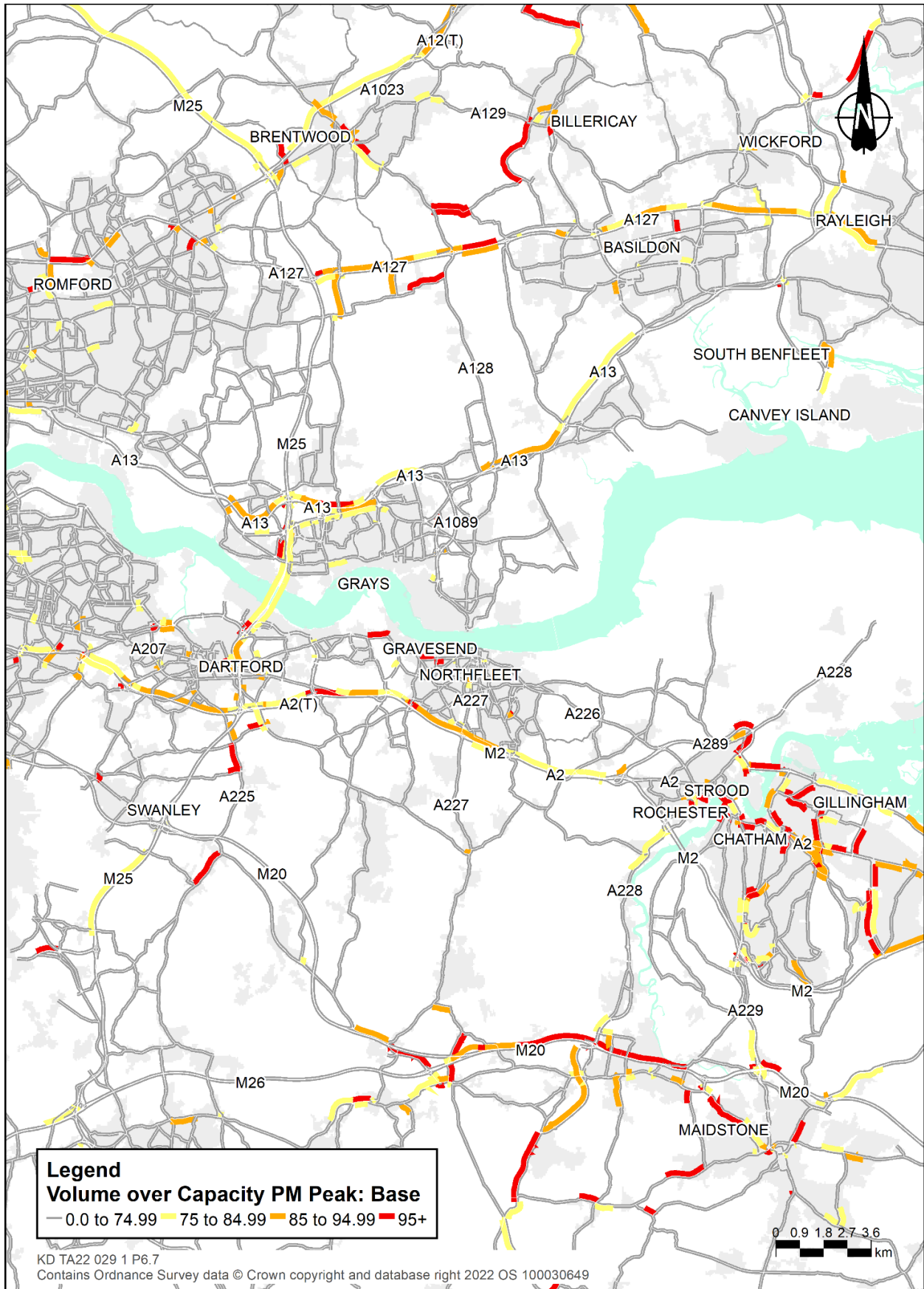
Plate 6.7 Volume to capacity 2016 PM peak (17:00-18:00)
